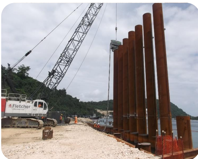
Pile Driving
